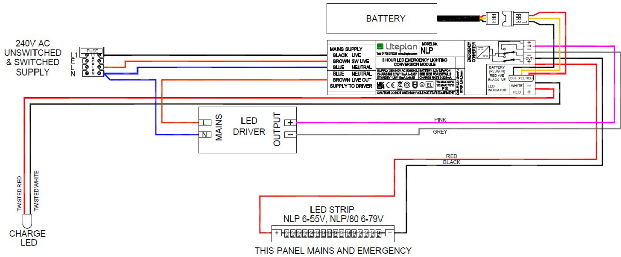
Typical Conversion Wiring Diagram
